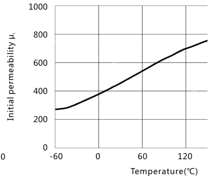
Initial permeability vs. Temperature
